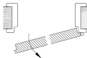
Right turning door Construction principal
