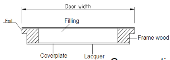
Cross section
