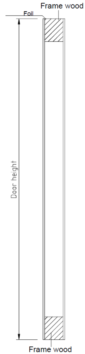
Cross section
