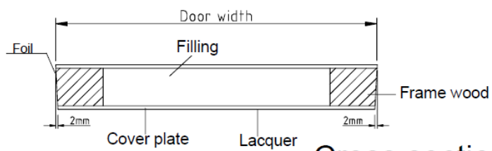
Cross section
