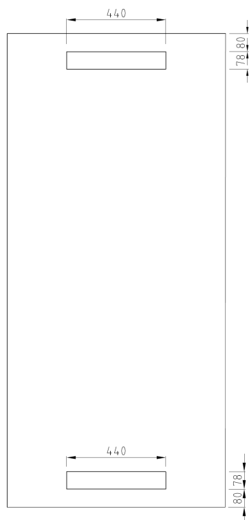
Vent – grate
