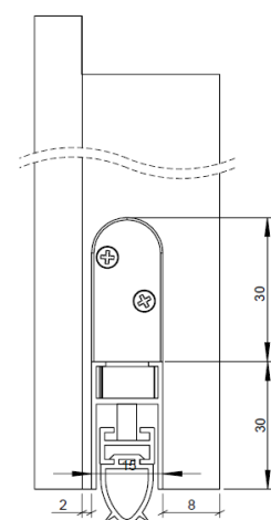
Groove for floor seal
