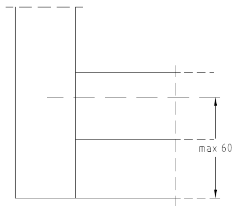
Shorten max 60 mm with double bottom rail
