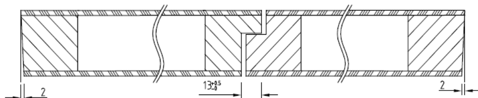
Double door flush with beveled edges and counter rebate
