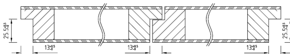
Rebate double door, with counter rebate
